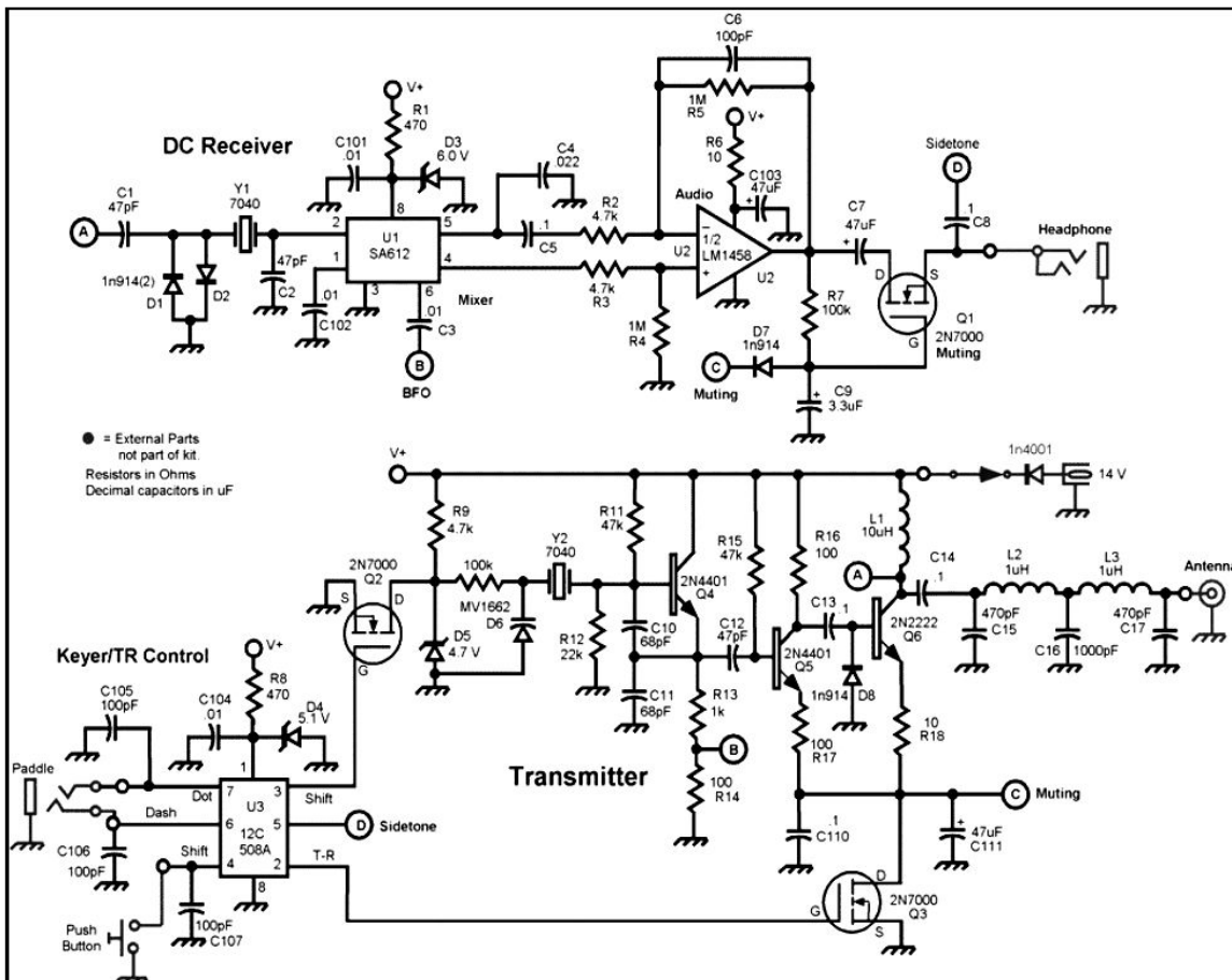
Rock-Mite/40 Schematic
